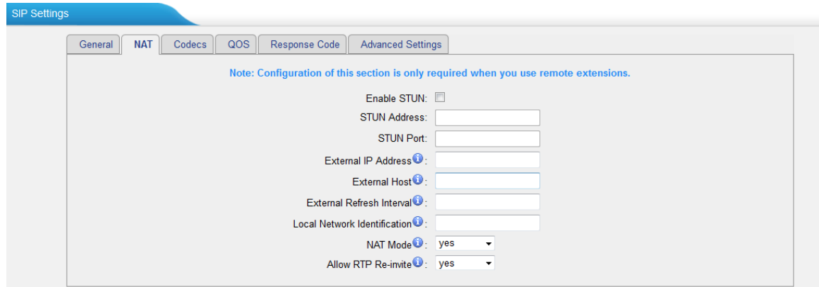
Figure 4-8 NAT Settings
