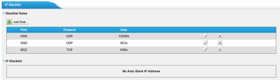
Figure 3-20 IP Blacklist
