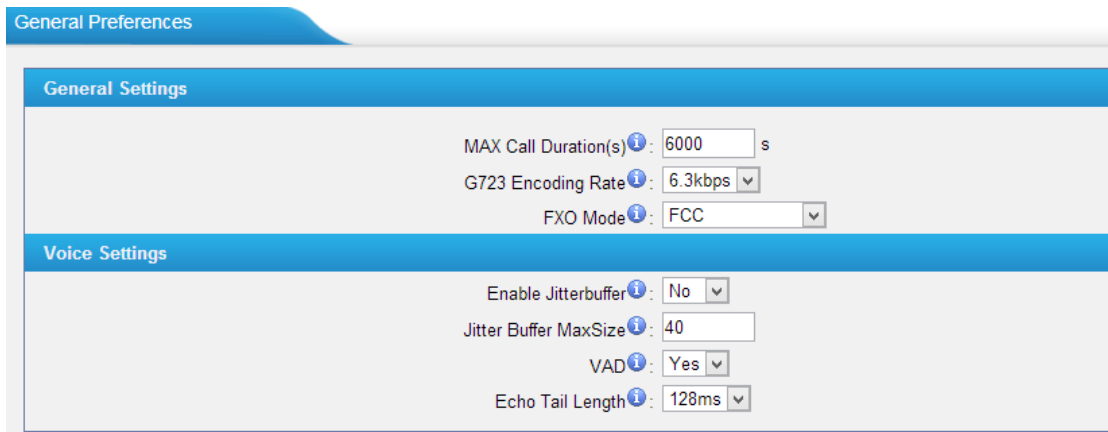
Figure 4-20 General Settings
