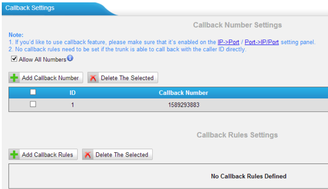
Figure 4-19 Callback Settings
