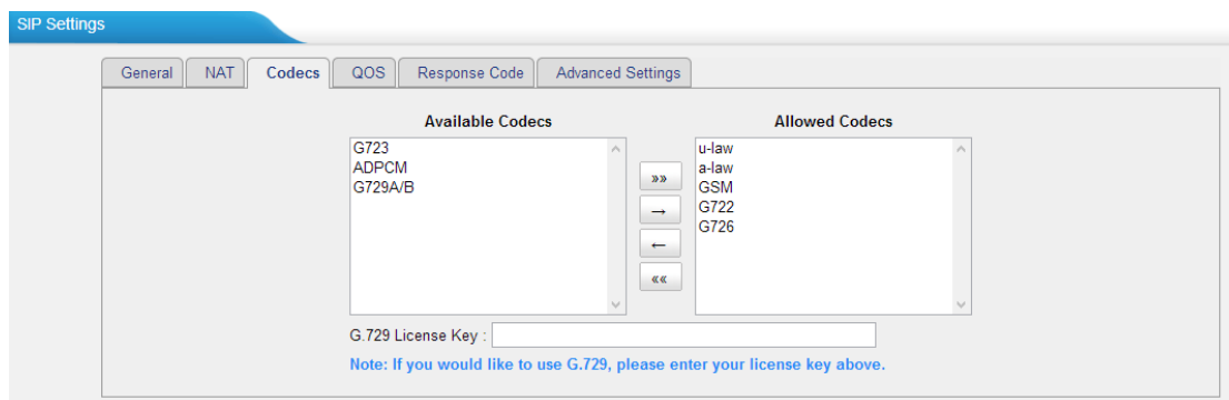
Figure 4-9 Codecs
