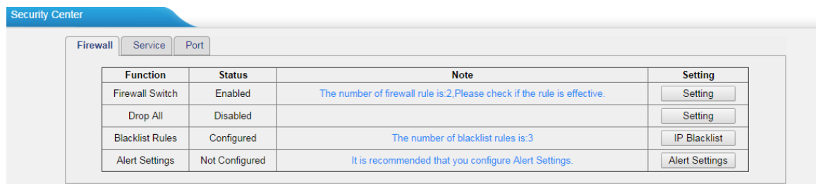
Figure 3-10 Firewall
