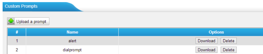
Figure 4-21 Custom Prompts
