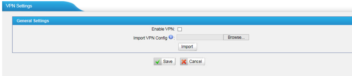
Figure 3-6 VPN Settings
