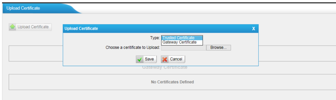
Figure 3-17 Certificates
