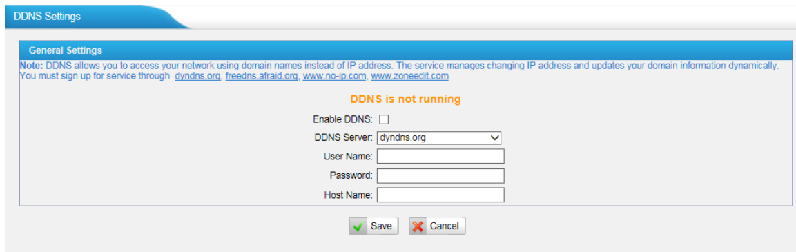
Figure 3-7 DDNS Settings
