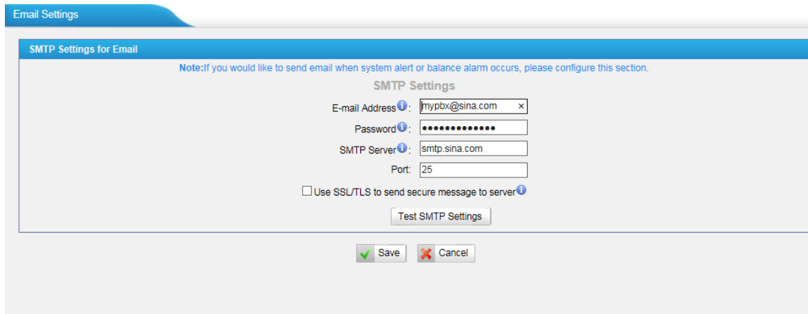
Figure 3-24 Email Settings
