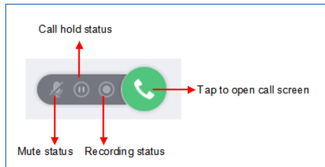
Figure 110: GAC2500 Web UI - Minimize Call Screen
