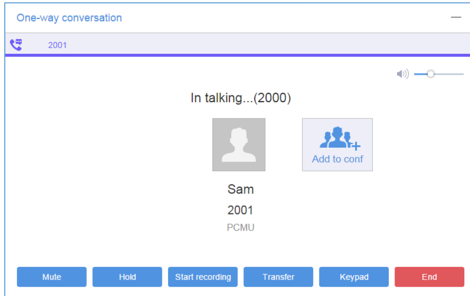
Figure 109: GAC2500 Web UI - Single Incoming Call
