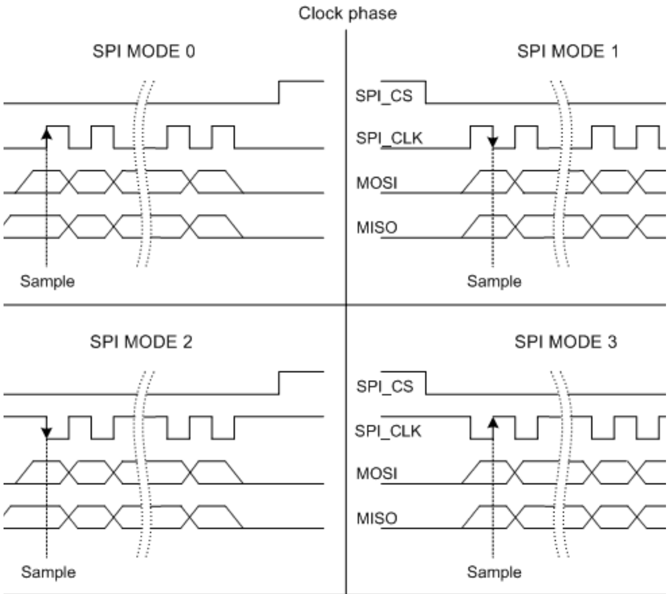
Figure 19.1: SPI modes selectable on SPI
